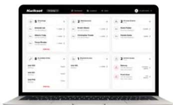
Desktop Portal
