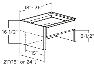
1 DRAWER 18"W - 36"W
