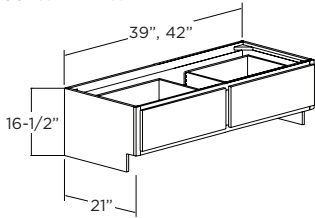
2 DRAWER 39"W - 42"W
