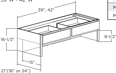
2 DRAWER 39"W - 42"W
