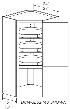
24" Wide Cabinet 20" Diameter Wood Lazy Susan Trays 27" Wide Cabinet 23" Diameter Wood Lazy Susan Trays
