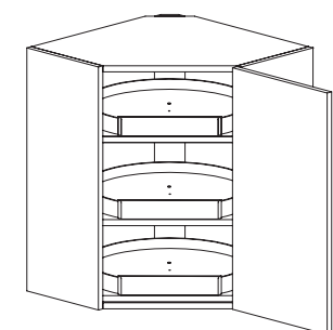
24" Wide Cabinet 20" Diameter Wood Lazy Susan Trays
