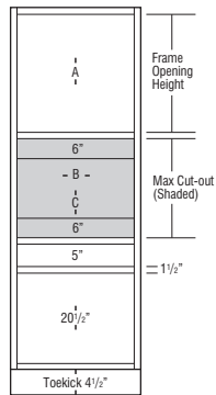
TBMWB _ _ _ 24N
