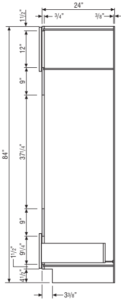
DOUBLE OVEN CABINET DEEP DRAWER
