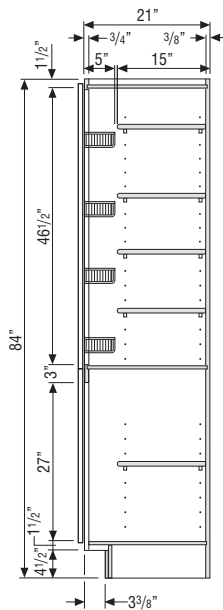
LCRH/LT CABINET (Aligns with 34 1/2" High Vanity Base Cabinets)
