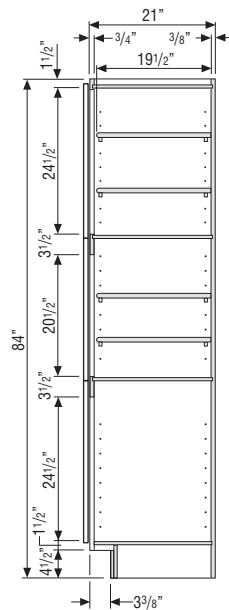
VANITY UTILITY CABINET (Aligns with 32" High Vanity Base Cabinets)
