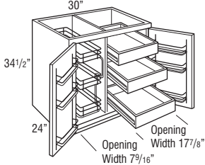
BSC30PR
