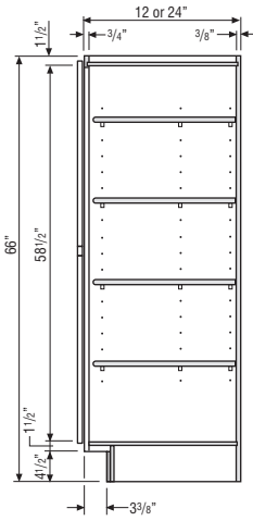
UTILITY CABINET
