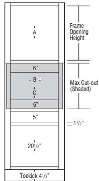
TBMWB _ _ _ 24
