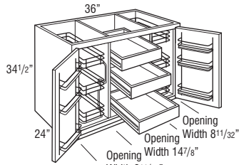
BSC36PRP
