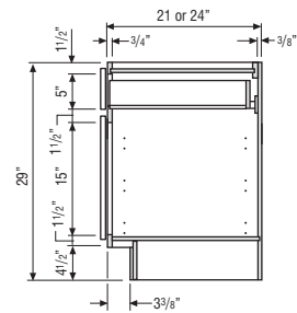
DESK BASE CABINET
