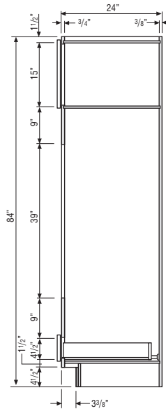
DOUBLE OVEN CABINET
