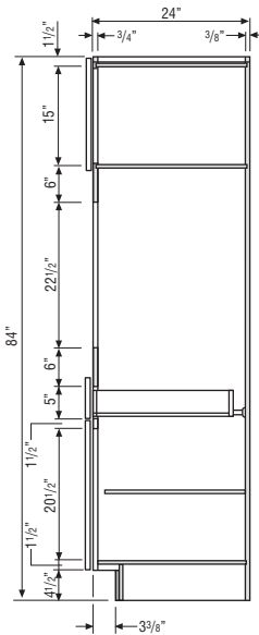
SINGLE OVEN CABINET
