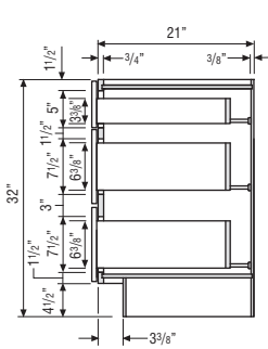
32" HIGH VANITY DRAWER BASE CABINET
